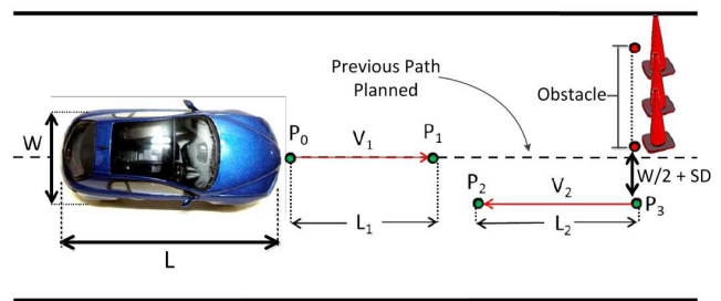
Fig. 4. Bézier control points generation in case of an obstacle avoidance maneuver (Beginning stage)
