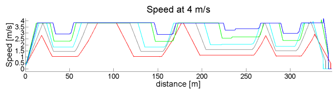
Fig. 9. Different speed profiles according to the levels implemented in [17]
