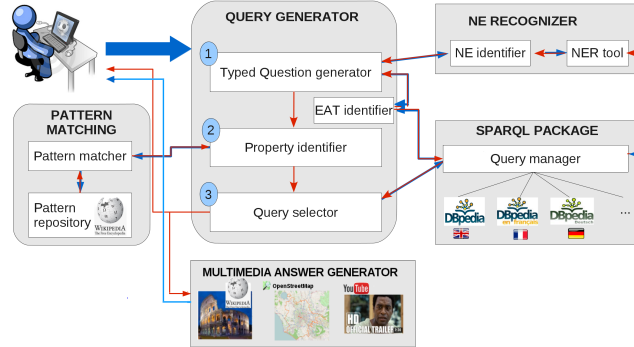
Fig. 1. QAKiS workflow [2]
