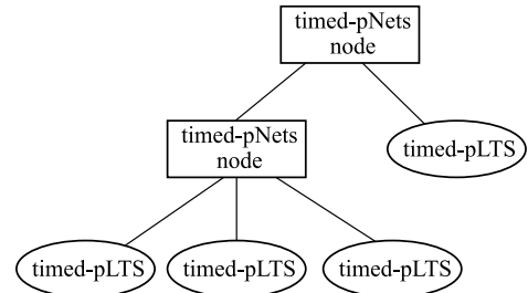
Fig. 1 Timed-pNets tree structure
