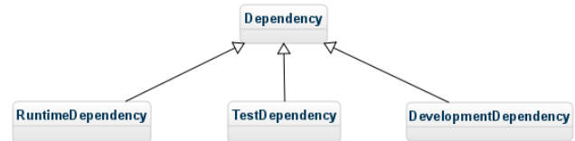
Figure 4. Dependency scopes
