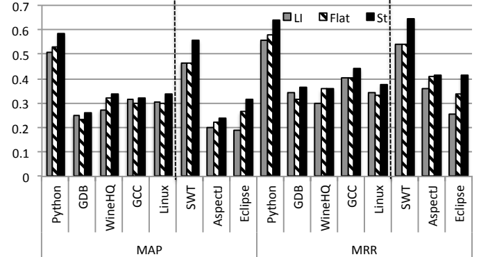
Fig. 4. Comparison of MAP and MRR for Different Strategies
