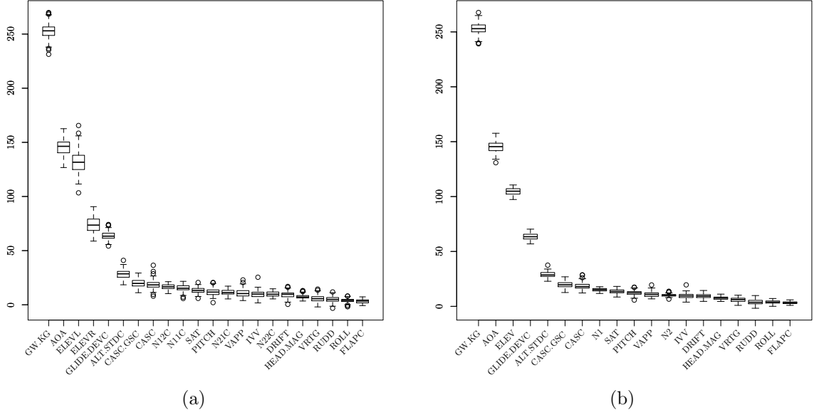
Figure 8: Application to long landing – Grouped variable importance measure before and after grouping the correlated flight parameters N11C and N12C, N21C and N22C, ELEVR and ELEVL into N1, N2 and ELEV.
