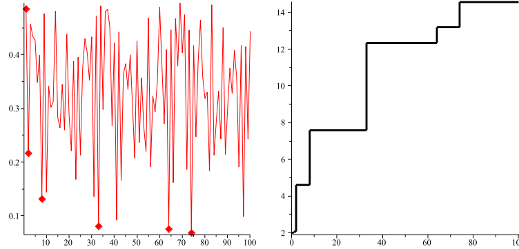
Fig. 3: Approximation function of p_1 = \cot(1) , p_2 = e^{-2} , and p_3 = 1 - p_1 - p_2 . Left: The quantities \| \{q\alpha^{(1)}\} \| , corresponding to \alpha^{(1)} = (1, w_2/w_1, w_3/w_1) and denominators q \in [1 \dots 100] , with BSADs rendered by diamonds. Right: the corresponding approximation function f_1 with jumps at the BSADs. (Data are for the sup-norm \| \cdot \|_\infty .)
