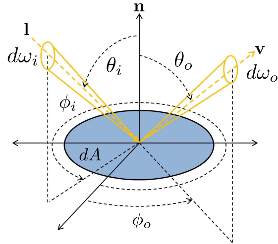
Fig. 1. The different vectors ( \mathbf{l}, \mathbf{v} ) and angles ( \theta_i, \phi_i, \theta_o, \phi_o ) used in this paper to parametrize the different BRDF models. The vector \mathbf{n} represents the surface normal and dA is the differential surface area on which the measurement with the detector is accomplished.
