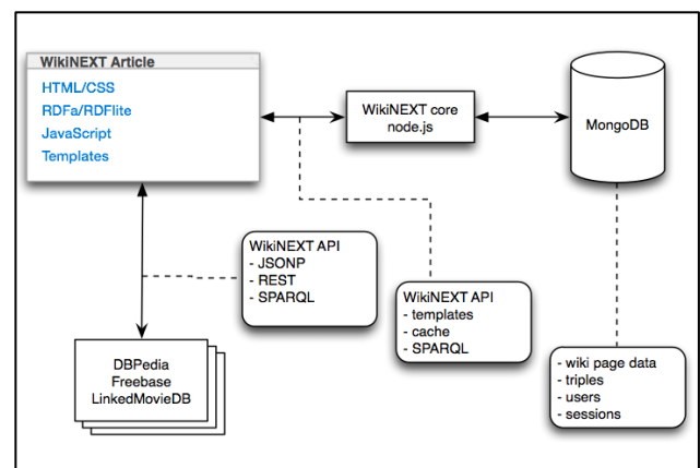
Figure 5: WikiNEXT Architecture.
