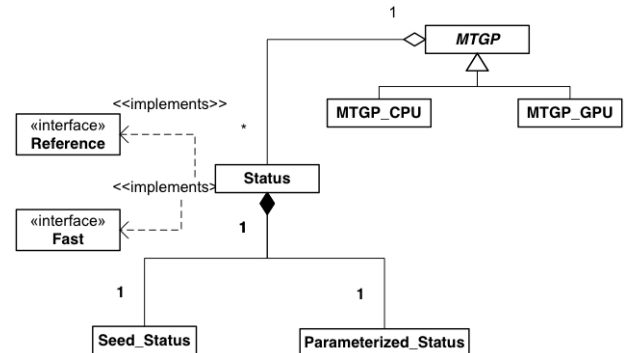
Figure 2: Class Diagram for MTGP and its components
