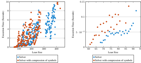
Figure 8. Solver Running Times.
