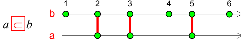
Figure 3: Example of subclocking. (For a sake of simplicity \chi(a)@r^\uparrow = 0 and \chi(b)@r^\uparrow = 0 )
