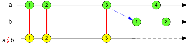
Figure 11: Examples of clock expression upto. (For a sake of simplicity \chi(a)@c^\uparrow = 0 and \chi(b)@c^\uparrow = 0 )
