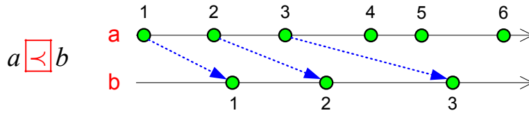
Figure 4: Example of precedence. (For a sake of simplicity \chi(a)@r^\uparrow = 0 and \chi(b)@r^\uparrow = 0 )
