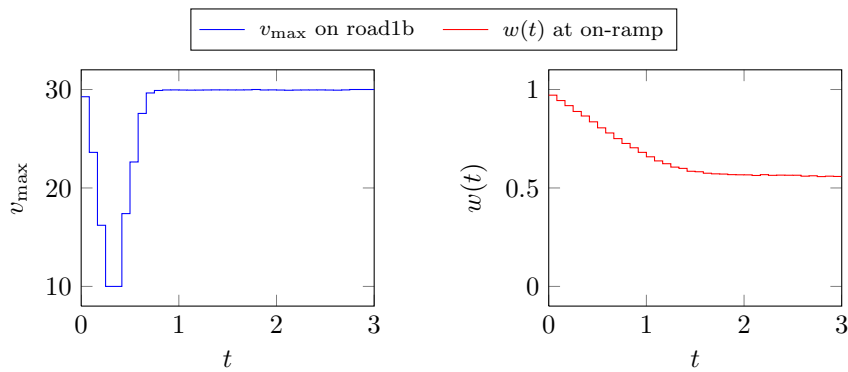
Figure 12: Optimal control of v_{\max} on road1b and w(t) at the on-ramp.
