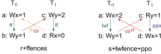
Fig. 16. The patterns r with full fences and s with lightweight fence and ppo (both forbidden).
