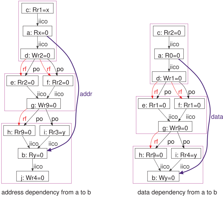
Fig. 23. Dataflow dependencies.
