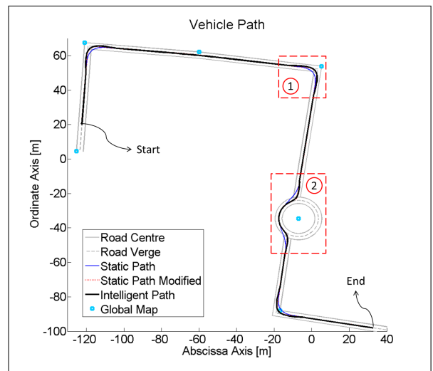
Fig. 5. Generated path
