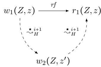
Figure 9: Assuming \xrightarrow{\star}_H^{i+1} is not causal
