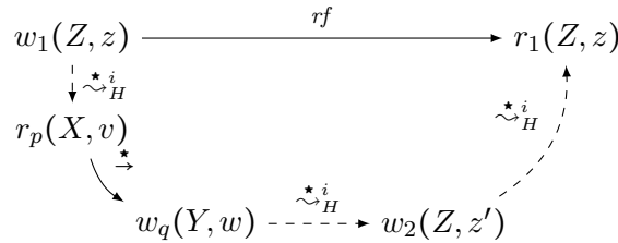
Figure 10: Assuming r_p(X, v) \xrightarrow{\star} w_q(Y, w) is only present in the path w_1(Z, z) \xrightarrow{\star}_H^{i+1} w_2(Z, z')
