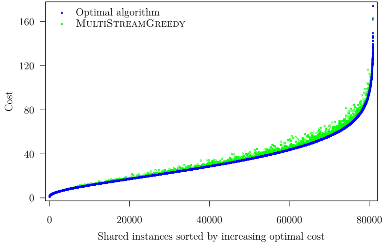
Figure 5: Cost achieved by MULTISTREAMGREEDY and that achieved by the optimal algorithm, shown for 81,000 random AND tree instances sorted by increasing optimal cost.
