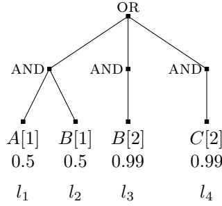
Figure 13: Example DNF tree for which the best schedule has larger cost than a non-linear strategy.
