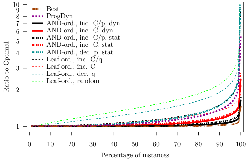
Figure 9: Ratio to optimal vs. fraction of the instances for which a smaller ratio is achieved, computed over 4,800 random “very small” DNF tree instances in the multi-stream case.
