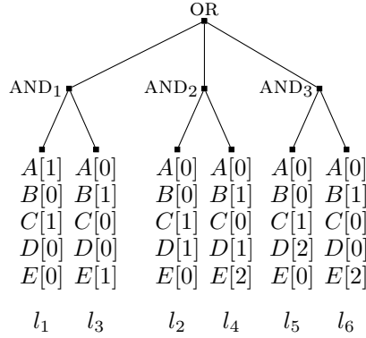
Figure 11: Example multi-stream DNF tree.
