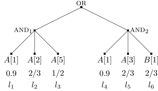
Figure 12: Example DNF tree for which SINGLESTREAMGREEDY does not produce an optimal schedule.
