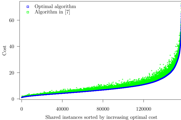
Figure 4: Cost achieved by the algorithm in [7] and that achieved by the optimal SINGLESTREAM-GREEDY algorithm, for 157,000 random AND tree instances sorted by increasing optimal cost.
