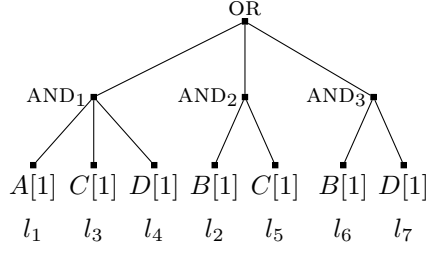
Figure 2: Example single-stream DNF tree.
