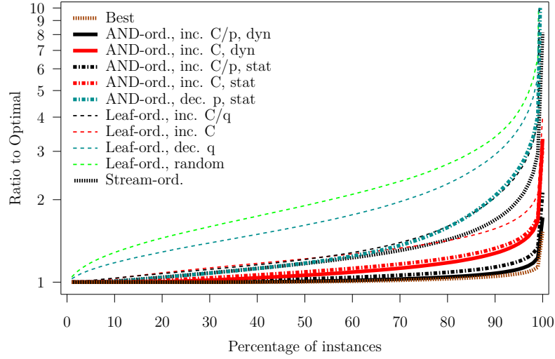
Figure 6: Ratio to optimal vs. fraction of the instances for which a smaller ratio is achieved, computed over 17,100 random “small” DNF tree instances in the single-stream case.
