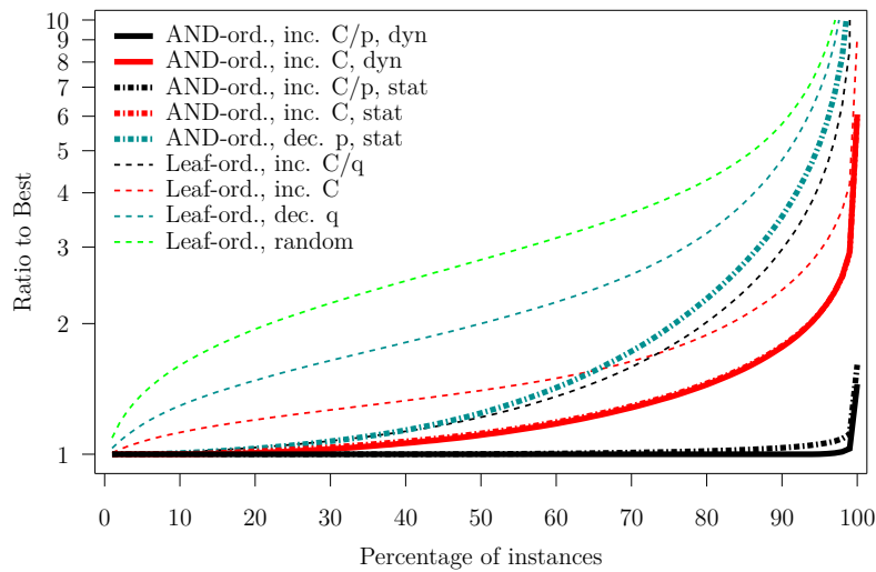
Figure 10: Ratio to the Best heuristic vs. fraction of the instances for which a smaller ratio is achieved, computed over 32,400 random “large” DNF tree instances in the multi-stream case.
