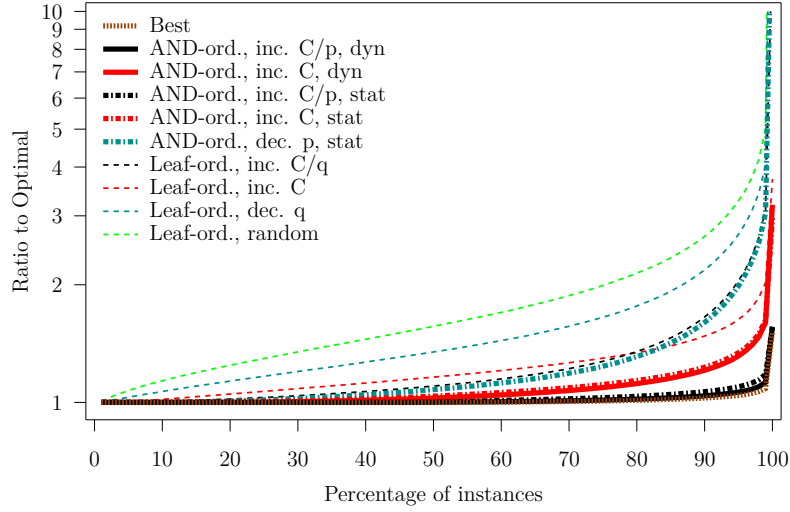
Figure 8: Ratio to optimal vs. fraction of the instances for which a smaller ratio is achieved, computed over 16,200 random “small” DNF tree instances in the multi-stream case.
