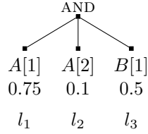
Figure 3: Example shared AND tree for which the read-once algorithm in [7] is not optimal.
