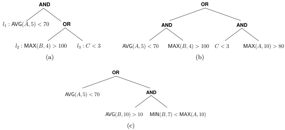
Figure 1: Three query tree examples: (a) a read-once query; (b) a shared query in the single-stream case; (c) a shared query in the multi-stream case.
