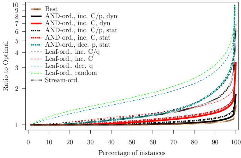
Figure 6: Ratio to optimal vs. fraction of the instances for which a smaller ratio is achieved, computed over 21,600 random “small” DNF tree instances in the single-stream case.
