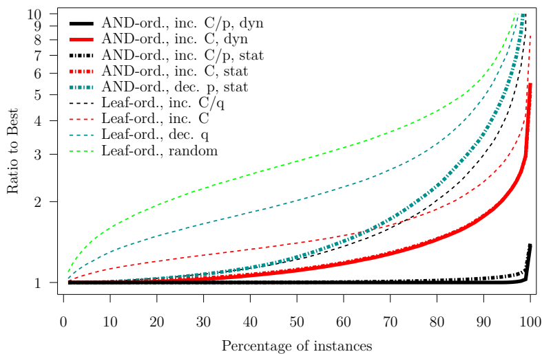
Figure 10: Ratio to the Best heuristic vs. fraction of the instances for which a smaller ratio is achieved, computed over 32,400 random “large” DNF tree instances in the multi-stream case.
