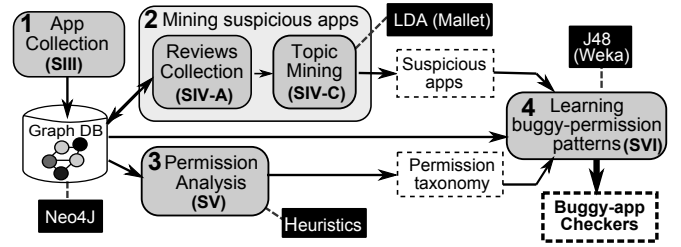
Fig. 1. Overview of our approach to identify efficient buggy app checkers.
