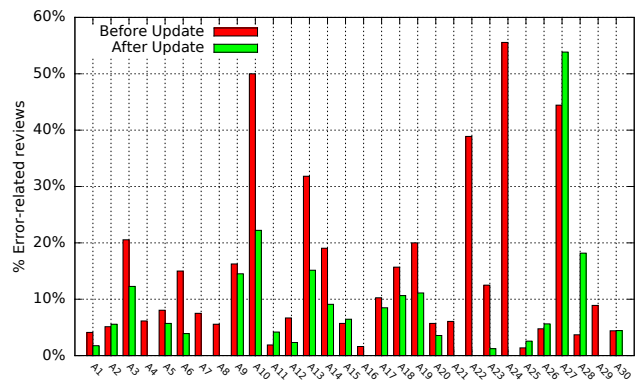
Fig. 8. Reviews evolution after removing error-sensitive permissions.
