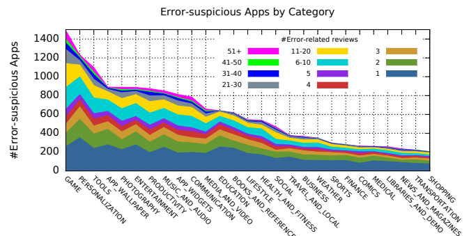
Fig. 5. Distribution of error-suspicious apps by categories in Google Play.
