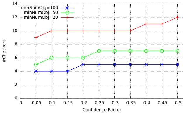
Fig. 6. Calibration of confidence factor and minNumObj parameters.
