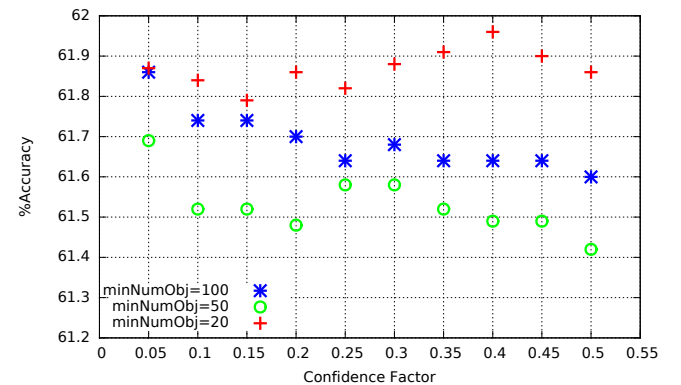
Fig. 7. Evaluation of the accuracy of the recommender system.
