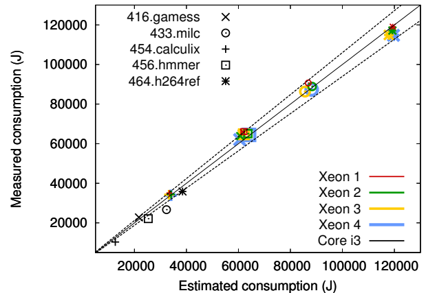
Figure 1: Energy consumption.
