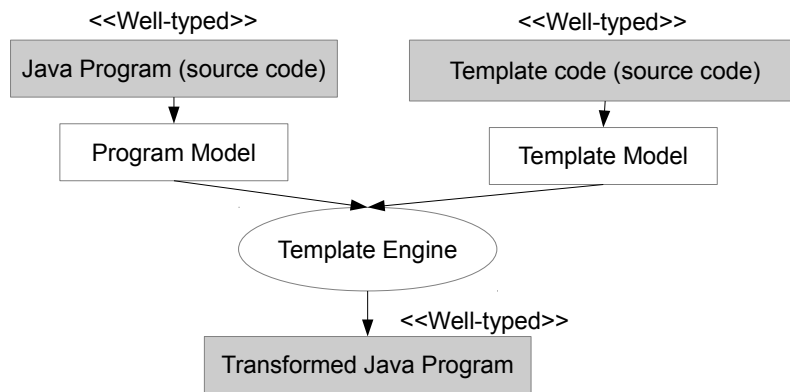
Figure 4: Overview of SPOON's Templating System.
