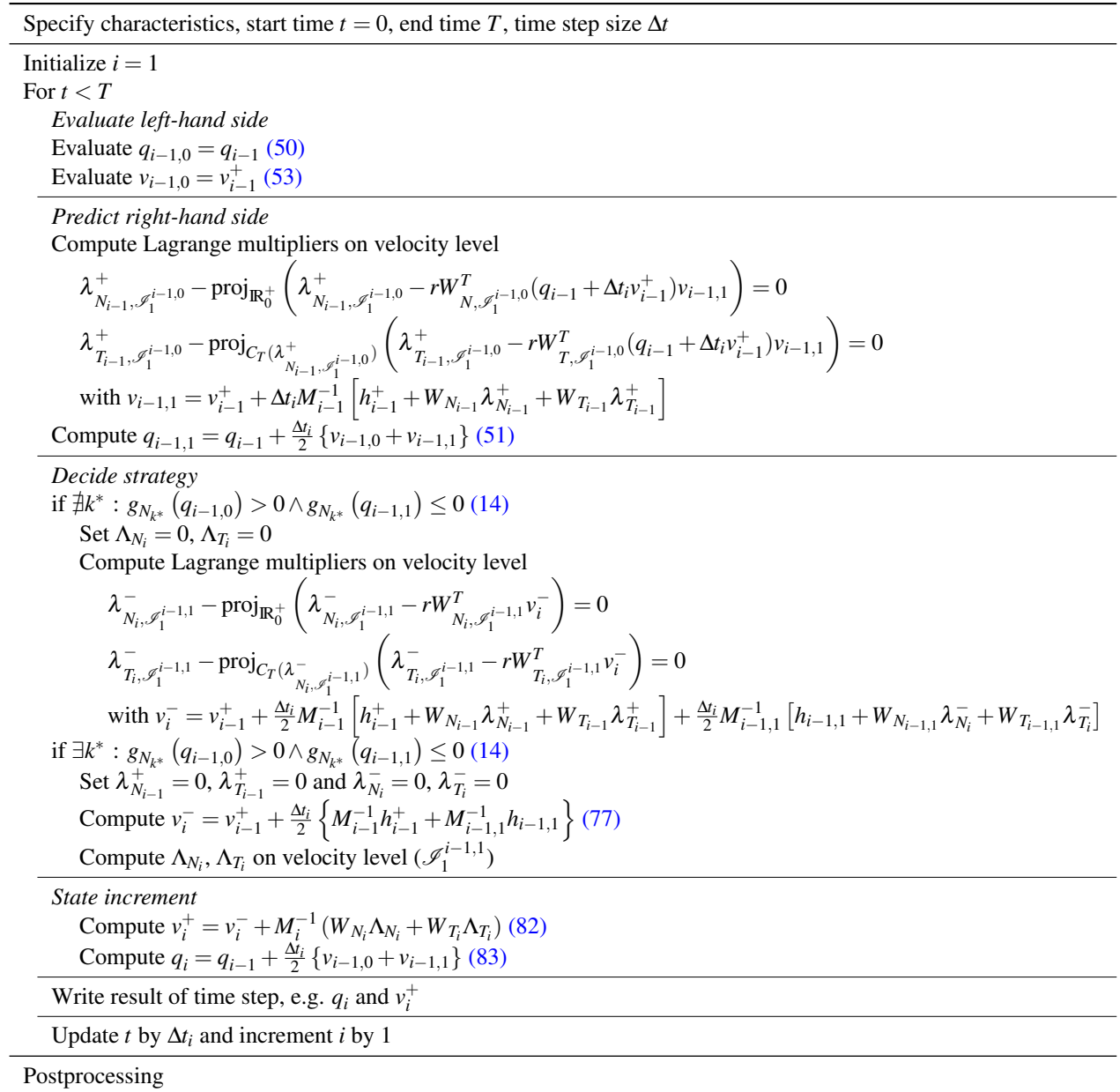
Figure 9: Flowchart of the half-explicit timestepping scheme on velocity level.
