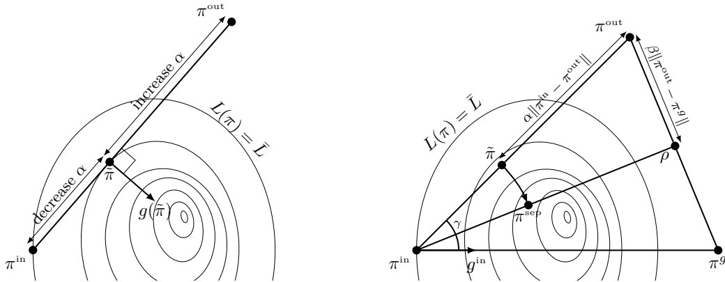
Fig. 5: Left: Auto-adaptive \alpha -schedule: condition for increasing or decreasing \alpha depending on whether the \pi^{\text{sep}} is below or beyond the threshold value \tilde{\pi} . Right: Directional Smoothing: combining sub-gradient and Wentges smoothing
