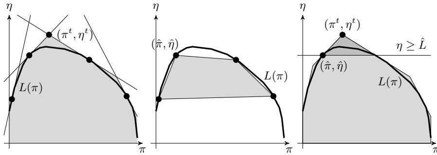
Fig. 1: Outer and Inner polyhedral approximation for the dual master polyhedron [DM] (10-12) and the trust polyhedra defined by adding a cut on the objective to the outer approximation.
