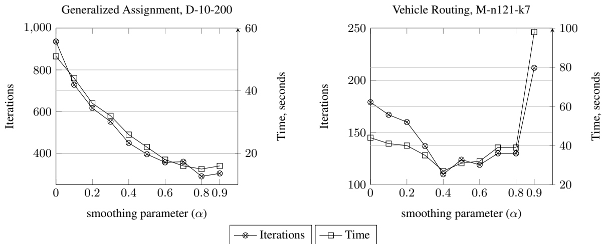
Fig. 8: Sensitivity of master iterations number and solution time to a static \alpha
