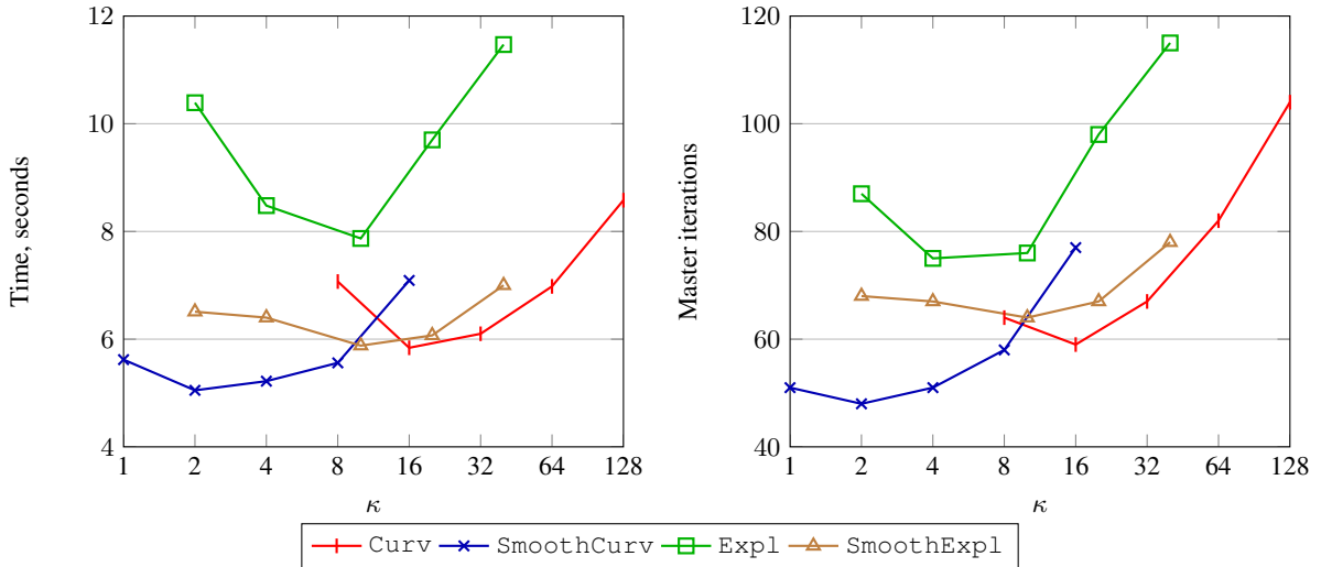
Fig. 10: Sensitivity of master iterations number and solution time to parameter \kappa for the Lot Sizing problem
