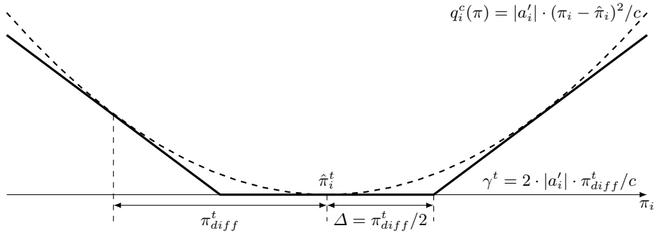
Fig. 7: Curvature based penalty function on iteration t
