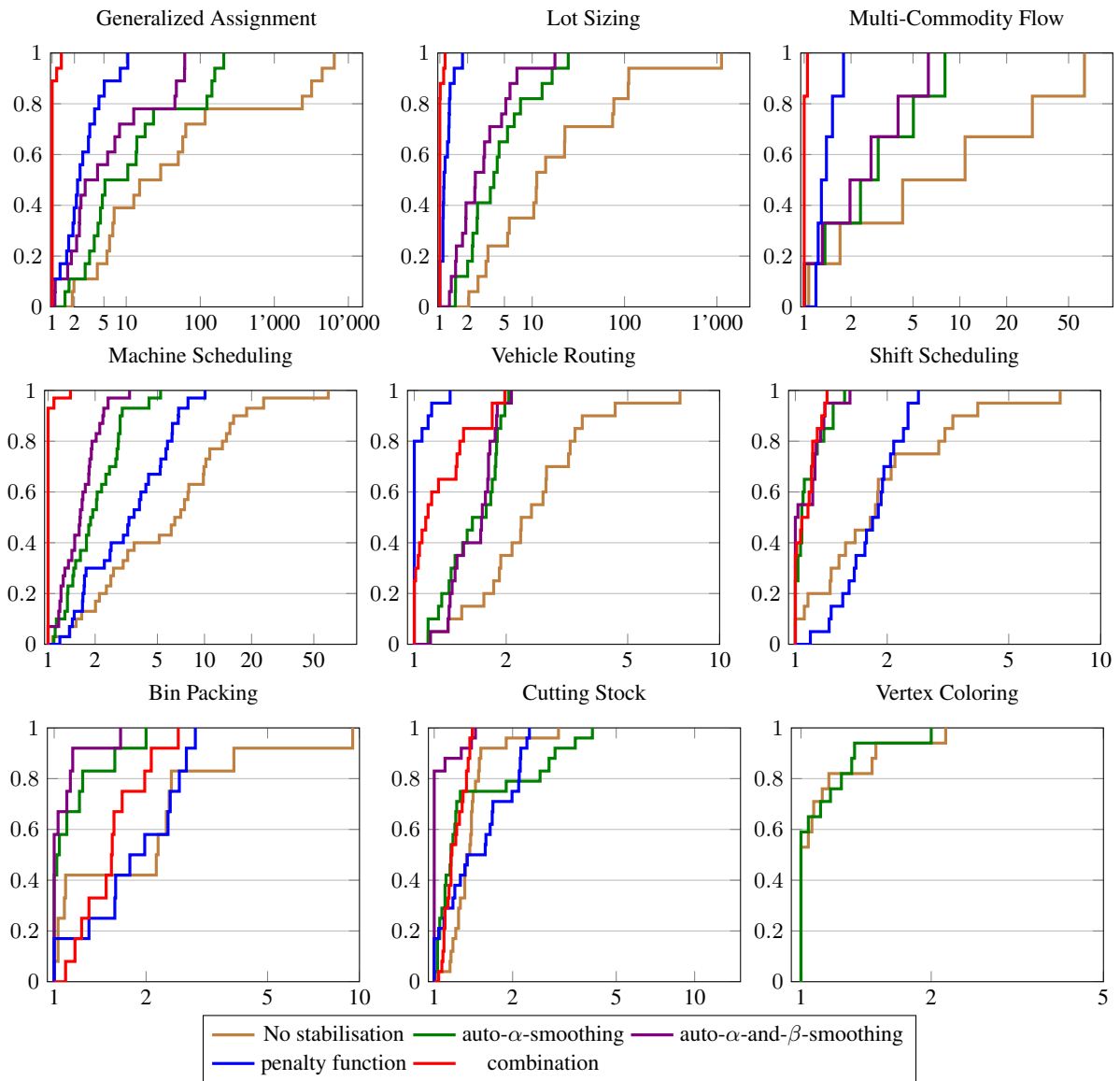
Fig. 11: Performance profile graphs
