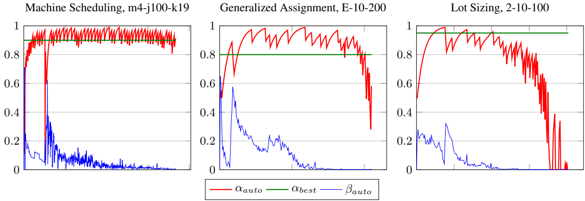
Fig. 9: Behaviour of values \alpha and \beta in the course of the column generation procedure using self-adjusting schemes
