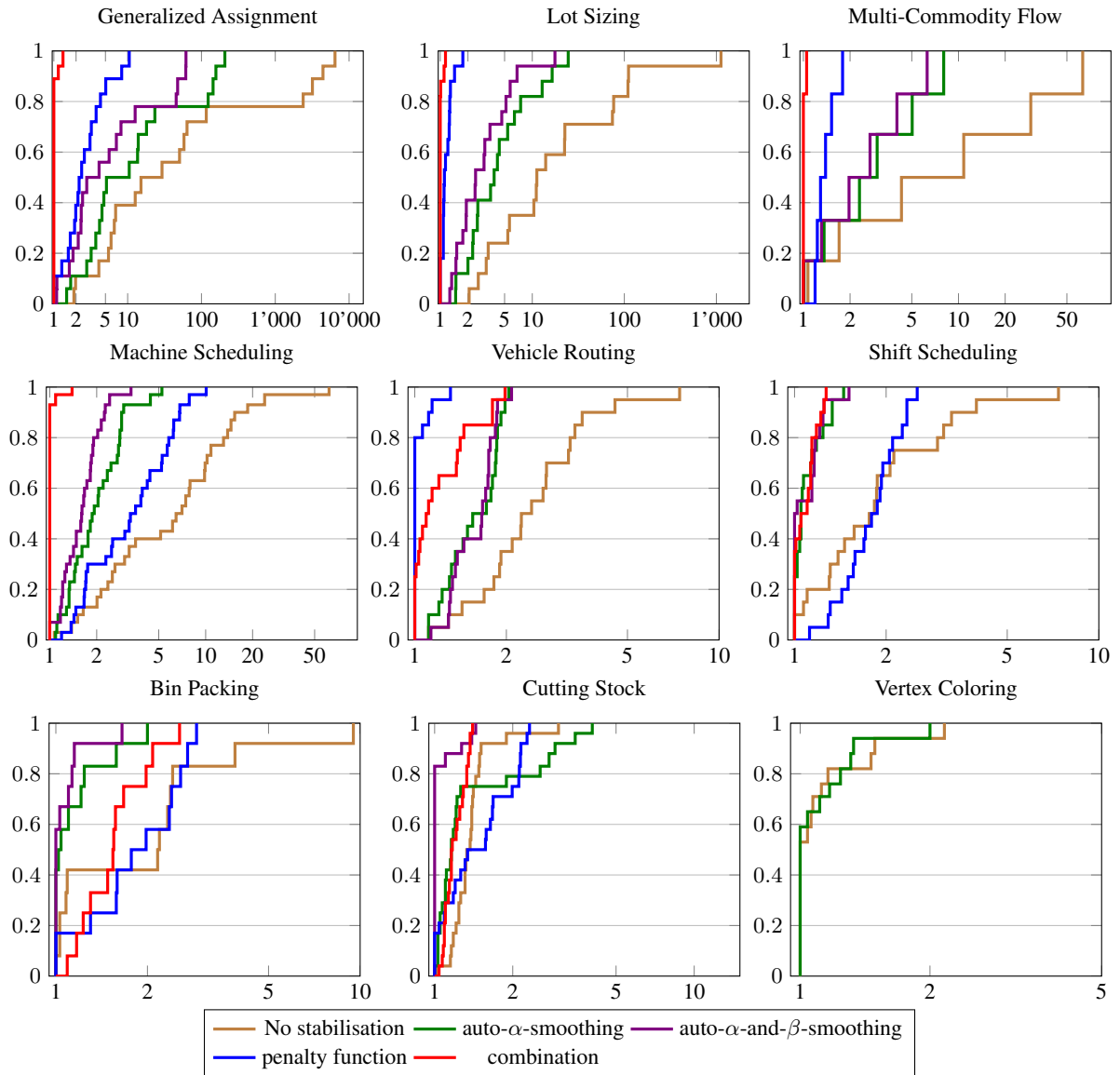
Fig. 12: Performance profile graphs
