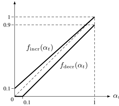
Fig. 6: Functions for increasing or decreasing \alpha
