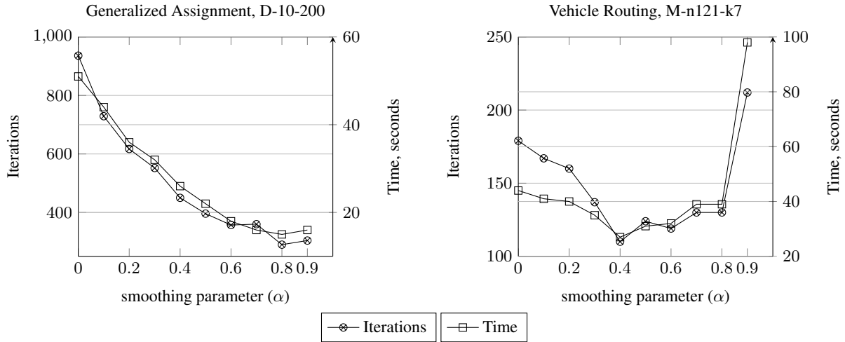
Fig. 9: Sensitivity of master iterations number and solution time to a static \alpha
