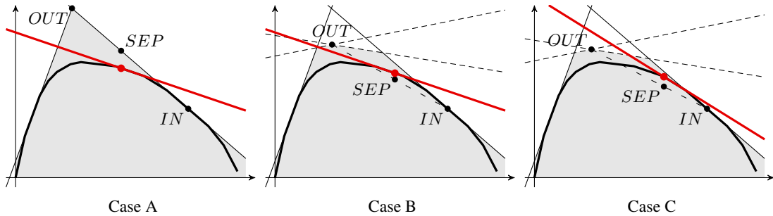
Fig. 2: The three cases that can arise when attempting to cut point (\pi^{sep}, \eta^{sep}) . Case A: (\pi^{sep}, \eta^{sep}) is cut-off by z^t , and hence so is (\pi^{out}, \eta^{out}) . Case B: (\pi^{sep}, \eta^{sep}) is not cut but (\pi^{out}, \eta^{out}) is. Case C: neither (\pi^{sep}, \eta^{sep}) , nor (\pi^{out}, \eta^{out}) are cut, which results in a mis-pricing .
