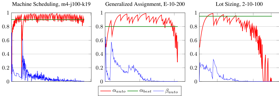
Fig. 10: Behaviour of values \alpha and \beta in the course of the column generation procedure using self-adjusting schemes
