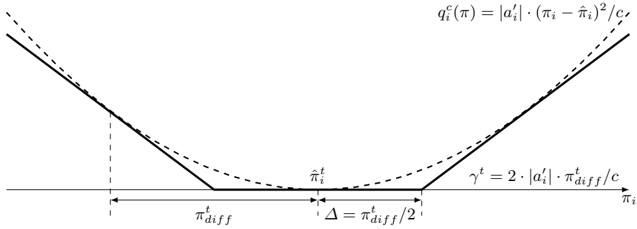
Fig. 8: Curvature based penalty function on iteration t
