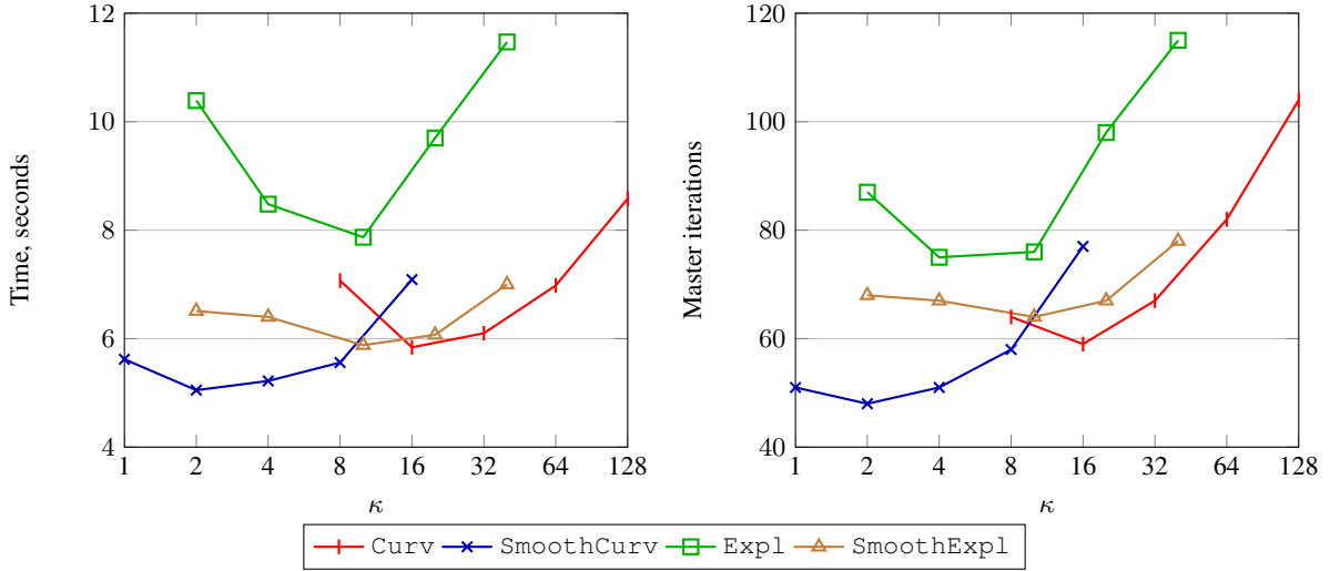
Fig. 11: Sensitivity of master iterations number and solution time to parameter \kappa for the Lot Sizing problem
