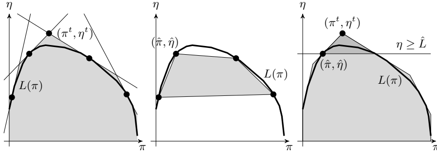
Fig. 1: Outer and Inner polyhedral approximation for the dual master polyhedron [DM] (10-12).
