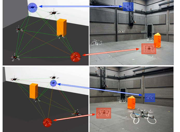
Fig. 6. Two snapshots of the reported experiment. Left: simulated 3D views showing, in particular, the inter-agent links (red – almost disconnected link, green – optimally connected link). Right: corresponding pictures of the experimental setup. The two highlighted quadrotor UAVs are partially controlled by two human operators
