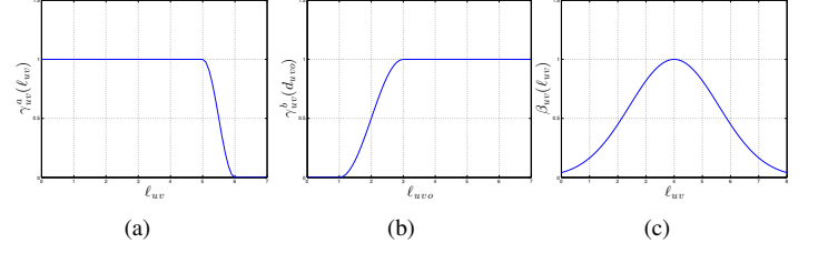
Fig. 3. The shape of \gamma_{uv}^a(\ell_{uv}) for D = 6 (a), \gamma_{uv}^b(\ell_{uvo}) for \ell_{\min} = 1 (b), and \beta_{uv}(\ell_{uv}) for \ell_0 = 4 (c).
