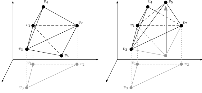
(a) Two equivalent minimally rigid frameworks in \mathbb{R}^3 . The framework on the right side is obtained by the reflection of the position of v_5 with respect to the plane characterized by the positions of v_1 , v_2 , and v_3 (as illustrated in grey).
