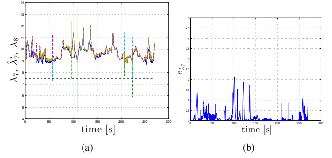
Fig. 8. Left: behavior of \lambda_7(t) (blue line) and the 6 estimations \hat{\lambda}_7^i(t) (dashed colored lines) which result almost coincident. Right: behavior of the overall rigidity eigenvalue estimation error e_\lambda(t) as defined in (35)
