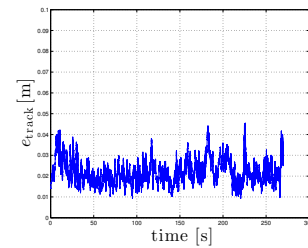
Fig. 12. Behavior of the tracking error e_{\text{track}}(t) defined in (36) showing again the good tracking performance of the 6 quadrotors
