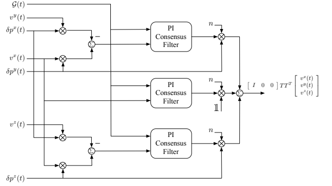
Fig. 5. Block diagram showing PI consensus filters in calculation of TT^T \hat{\mathbf{v}}(t) .
