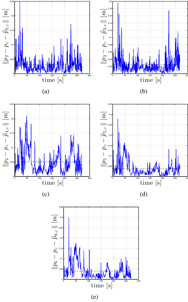
Fig. 7. Behavior of \|p_i - p_c - \hat{p}_{i,c}\| , i = 2 \dots 6 , the norm of the estimation error for the relative positions of agents 2 \dots 6 w.r.t. agent i_c = 1 . The horizontal dashed black line represents the mean value of each error norm over time. Note how the estimation errors keep a low value during the group motion and thus indicate the ability of each robot to recover its relative position with respect to the robot i_c = 1 by only exploiting measured distances with respect to its neighbors and the infinitesimal rigidity of the formation
