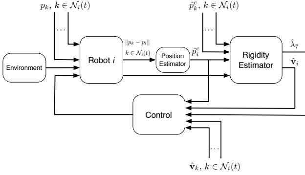
Fig. 4. Control architecture for distributed rigidity maintenance.
