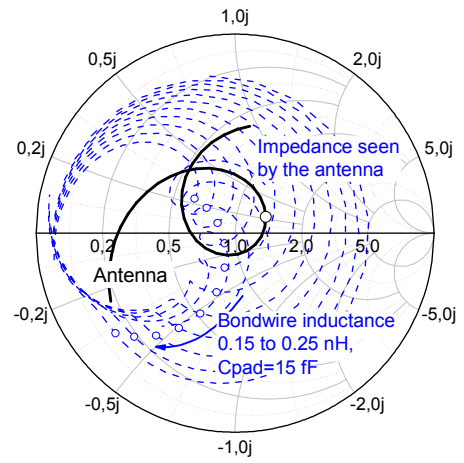
Fig. 3. Matching strategy of the LCL interconnect depicting the impedance at the antenna reference plane. The blue dashed lines show the impedance across 110-150 GHz band seen by the patch antenna for different values of the bondwire inductance. Circles highlight the mid-band (130 GHz).
