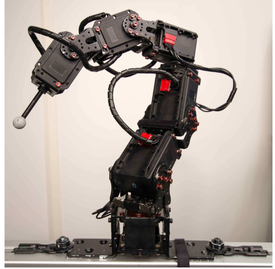
Fig. 2. Our robots sports 3 RX-64 servomotors from the base, then 3 RX-28 and a reflective marker at the tip.
