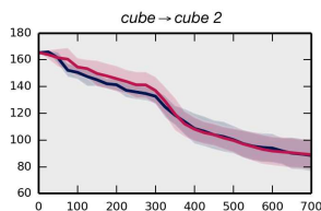
Fig. 6. Even in situations where is it not useful, the reuse is not detrimental to the learning performance. Averaged error over 10 repetitions.
