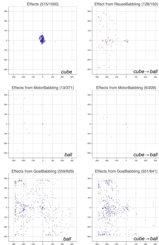
Fig. 7. The reuse of exploration trajectories can shape development. Here, the ball is learned to be moved predominantly on the left in cube \rightarrow ball , compared to the unperturbed task ball . The cube source task displays a bias towards left effects, and produces skewed reuse observations in the cube \rightarrow ball task, that have a lasting impact on the exploration. The number of salient effects versus the total number of interactions is indicated for each graph.
