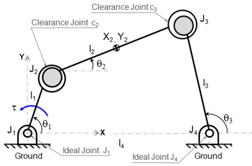
Figure 1: Four-bar mechanism with two imperfect revolute joints
