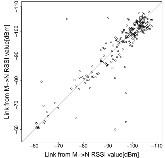
Figure 3: Symmetry of existing bidirectional links
