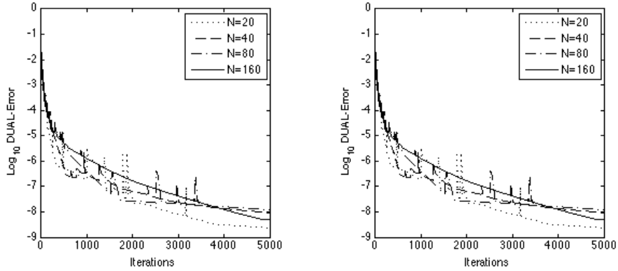
FIGURE 6. Test cases 1 (left) and 2 (right) : Convergence history of \log_{10}(\text{DUAL\_Error}) versus ALG2 iterations and N = 20, 40, 80, 160 .
