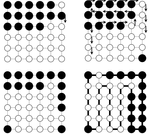
Fig. 5: Algorithm to achieve S^* from \mathcal{C}^* .
