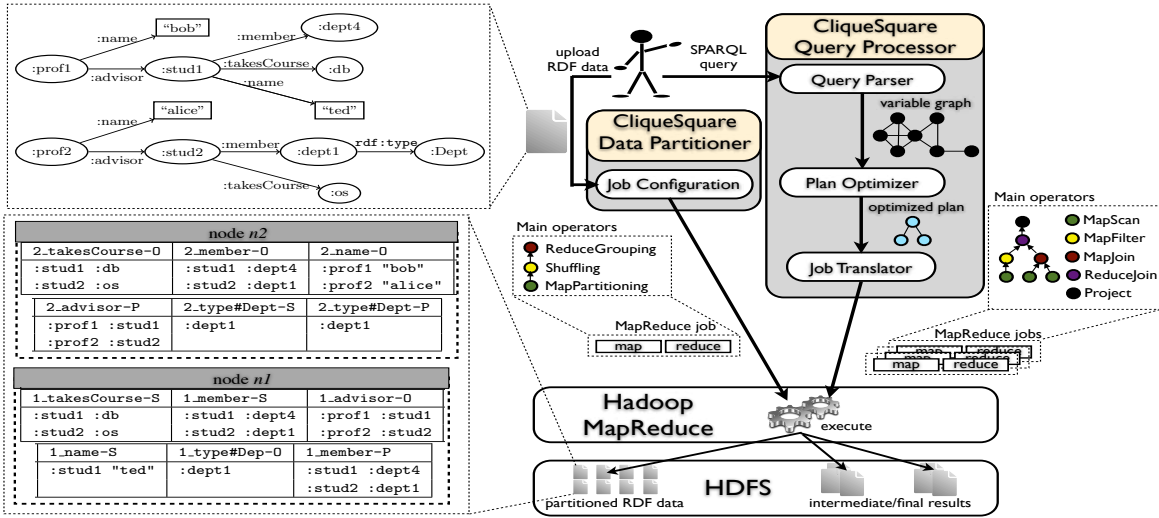
Figure 1: CliqueSquare architecture.
