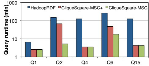
Figure 3: Query evaluation time for LUBM20K.
