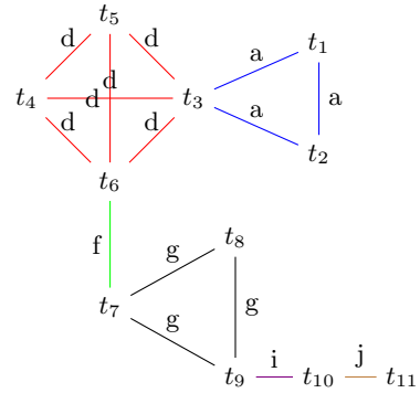
Figure 2: Query Q_1 and its variable graph G_1 .
