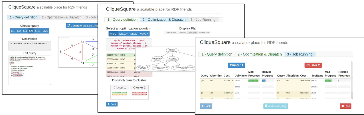
Figure 4: Cliquesquare graphical user interface.
