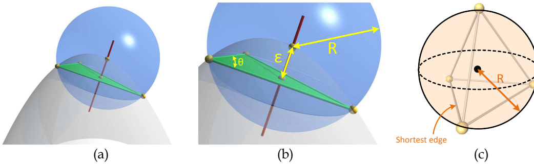
Fig. 5. (a) Surface Delaunay ball. (b) Surface Delaunay ball radius ( R ), approximation error of the surface ( \epsilon ) and triangle angles (e.g. \theta ) are used by the facet criteria. (c) Circumsphere radius ( R ) and shortest tetrahedron edge are used by the cell criteria.
