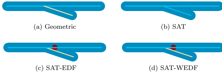
Fig. 15 Comparison of Algorithm Results. (a) The Geometric Algorithm, (b) The SAT, (c) EDF-Adjusted SAT with EMA in red, (d) WEDF-Adjusted SAT with WEMA in red.
