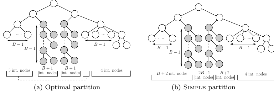
Figure 1: Optimal partition and the SIMPLE partition. The number of internal nodes (int. nodes) per bin is shown to facilitate the computation of the total node dispersal number.
