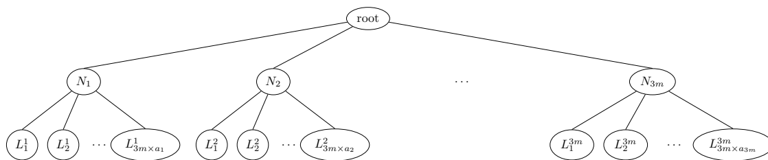
Figure 1: Tree used for the NP-completeness proof
