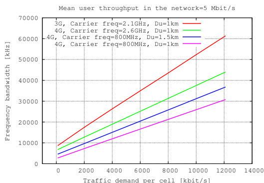
Fig. 6. Bandwidth versus traffic demand per cell to assure a mean user's throughput in the network \bar{r} = 5\text{Mbit/s} .
