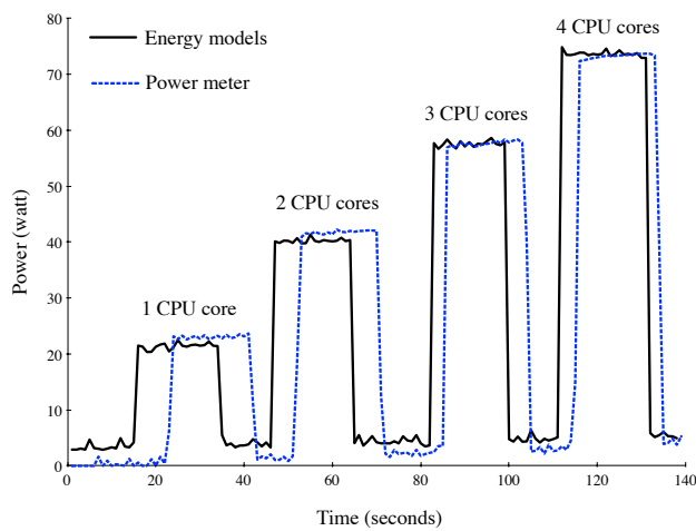
Fig. 7 Stressing the processor cores with the STRESS command.
