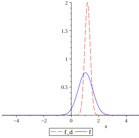
Fig. 3: Ornstein-Uhlenbeck (state)
