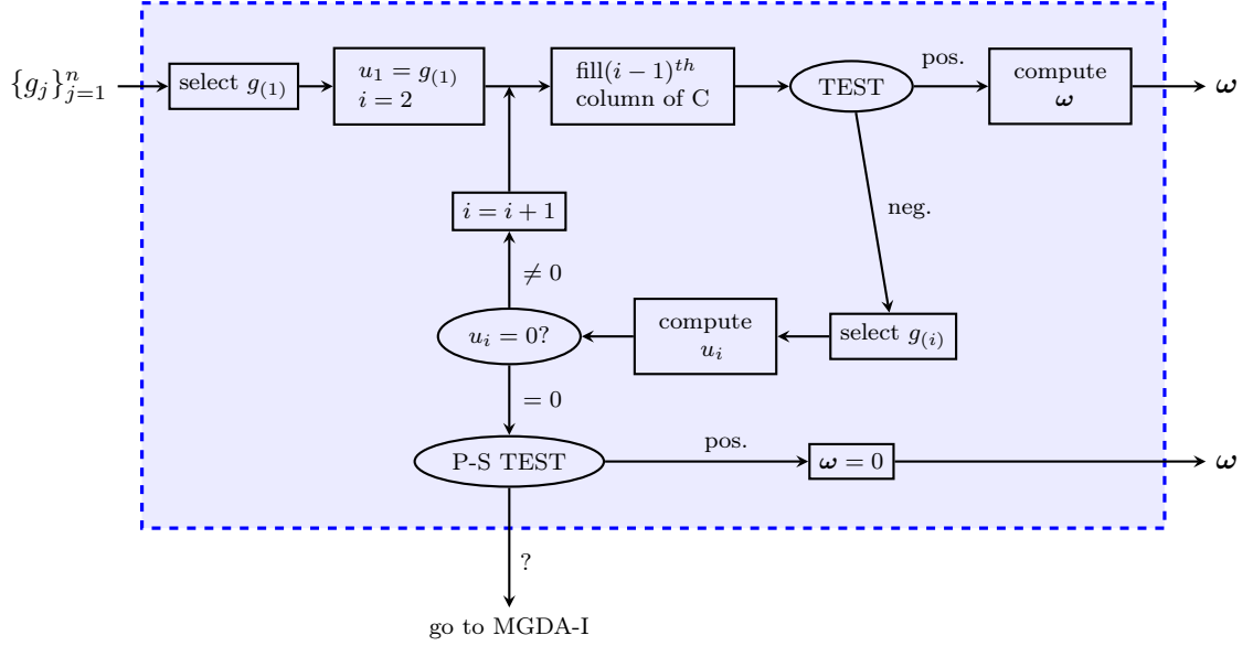
Figure 7: Flow chart of third version of MGDA
