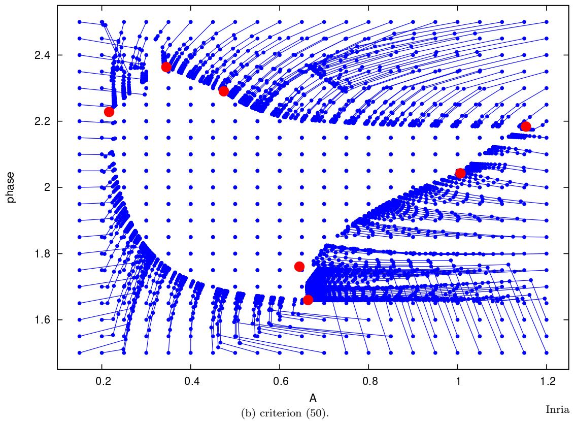
Figure 22: Result of MGDA applied to the nonlinear case from different starting points.
