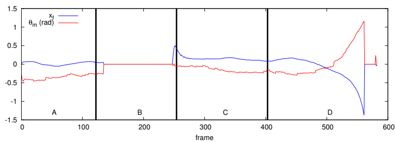
Figure 15: The evolution of the corridor visual features x_f and \theta_m
