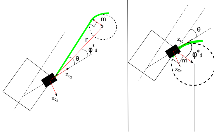
Figure 8: The desired camera trajectory shown in green. (a) when r > m and (b) when r < m .
