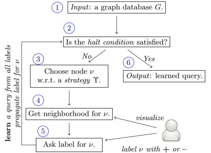
Figure 9: Interactive scenario.
