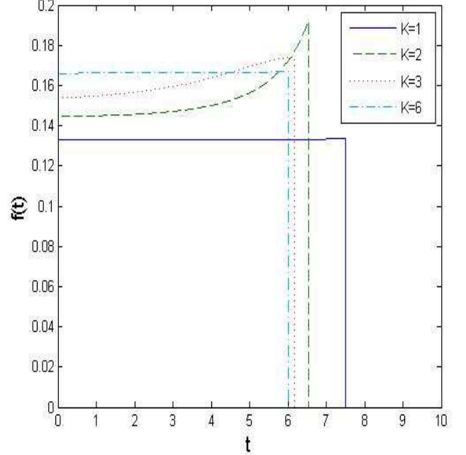
Fig. 1: Equilibrium density functions.
