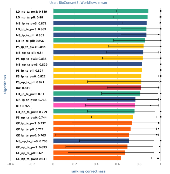
Fig. 5: Mean ranking correctness (bars) with upper and lower stddev (errorbars), and mean ranking completeness (black squares) over 24 lists of 10 workflows for different algorithms and configurations (see Table I for notation).
