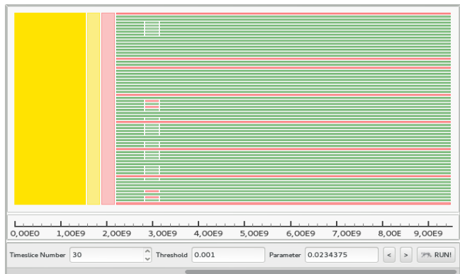
Figure 2. Ocelotl showing an overview of the execution of the NAS-CG application, class C, 64 processes, on the Grid'5000 Rennes site. The trace is partitioned into aggregates that correspond to a locally homogeneous behavior of the application over time and among a set of computing resources. We distinguish a perturbation around 3,00E9, caused by the concurrent execution of applications competing for network access.
