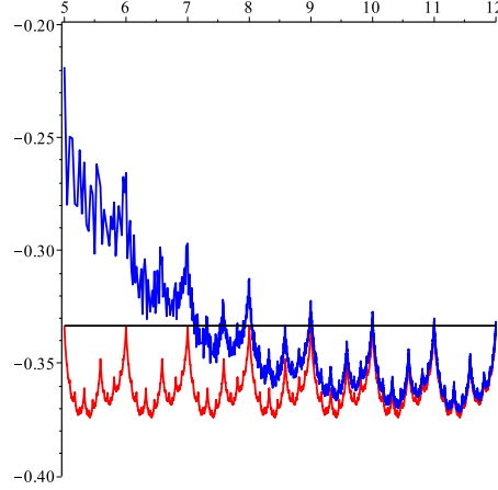
FIGURE 2. Theory is closely akin to practice: for the dichopile algorithm, the normalized sequence N^{-1}(f_N - N \log_2(N)/2) approaches the 1-periodic function \varphi(t) as N goes towards infinity. Abscissæ are in logarithmic scale for N . The maximum value of the periodic function is -1/3 .
