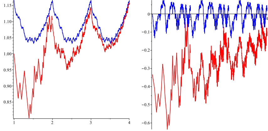
FIGURE 6. From Example 12, on the left, the periodic function \varphi_{2/3}(t) and the sequence s_N/N^{2/3} ; on the right, the periodic function \varphi_{1/3}(t) and the sequence (s_N - N^{2/3}\varphi_{2/3}(\log_8 N))/N^{1/3} .
