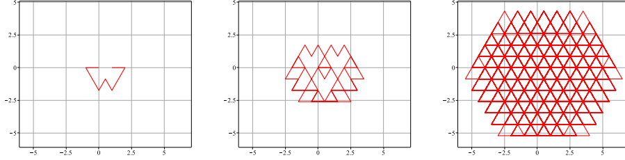
FIGURE 3. The image of the parameterized curve \mathbf{s}_K(x) from Ex. 7 grows linearly with K . Here we see \mathbf{s}_3 , \mathbf{s}_6 , and \mathbf{s}_{12} .
