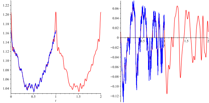
FIGURE 7. For both functions \varphi_{2/3}(t) (left) and \varphi_{1/3}(t) (right) from Example 12, their graph computed by the cascade algorithm (between 0 and 1) and by the partial sum of their Fourier series with twenty harmonics (between 0 and 2).
