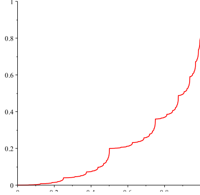
FIGURE 4. Limit probability distributions which come from a Bernoulli process described in Ex. 8.
