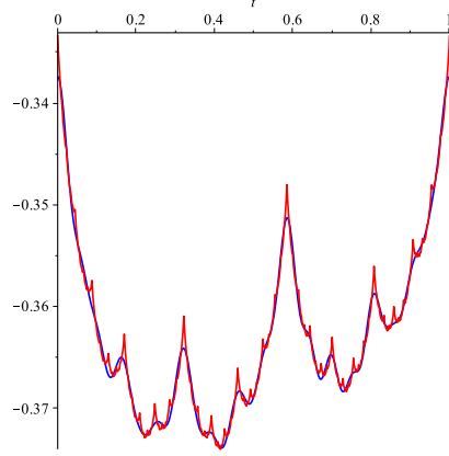
FIGURE 8. The periodic function \varphi(t) of the dichopile algorithm and its Fourier sum of order 10.
