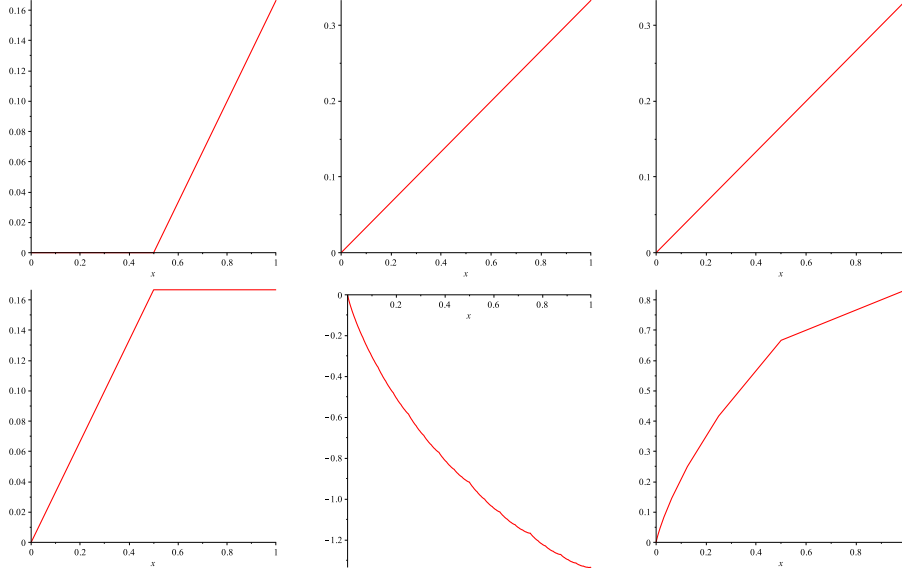
FIGURE 1. The six components (from left to right, and from top to bottom) of the vector-valued function \mathbf{g}(x) = \mathbf{f}^{(1)}(x) for the dilation equation associated with the dichopile algorithm.
