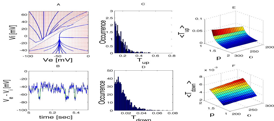
Figure 1. Bi-stability in a simplified neural-mass version of the Hutt & Longtin model [2], with neuron firing rates functions of Heaviside kind. A. 2D phase-portrait in the PSPs membrane potentials, showing the vector field (arrows) and sample free-noise trajectories (blue) that converge to either of two existing attractors. An oblique line, containing unstable (saddles) states, largely separates the attraction basins. B. Noise-induced alternations between a larger ( up state) and a smaller ( down state) value can be tracked according to the current distance of the trajectory to the saddle line. C, D. Histograms of the residence times in each of the stable states. E, F. The mean residence times as a function of the propofol level ( p ) and the inverse of the excitatory synaptic impulse response time-scale ( \alpha ).
