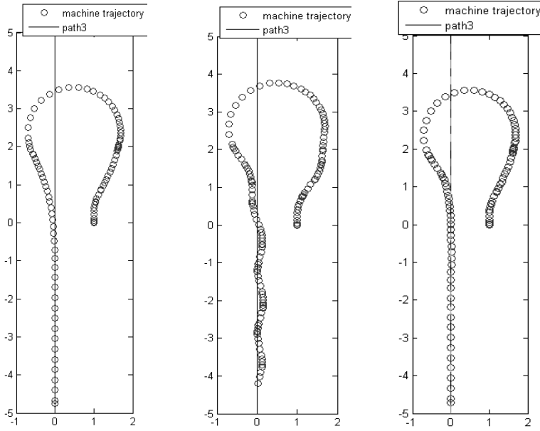
(a): Simulation result of headland turning control with fixed look-ahead 1m
