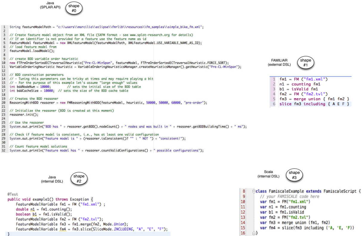
Figure 2. An example of SPLAR API and three polymorphic variants of the same domain-specific code snippet
